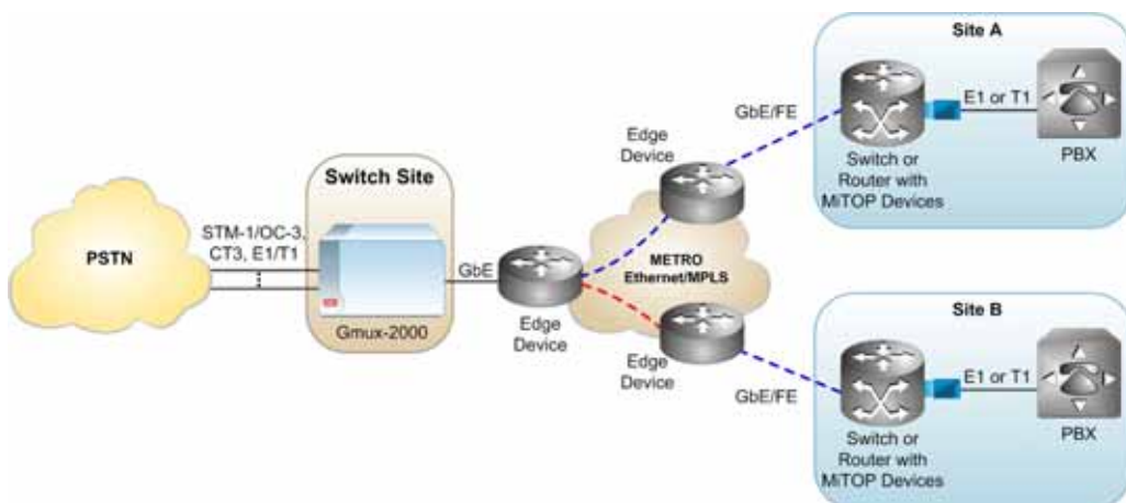
Figure 1. Aggregating TDM Services over PSN
