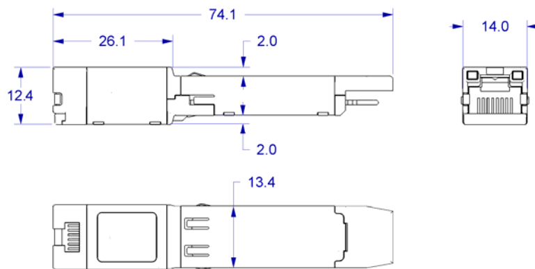
Figure 2 Physical Dimensions
