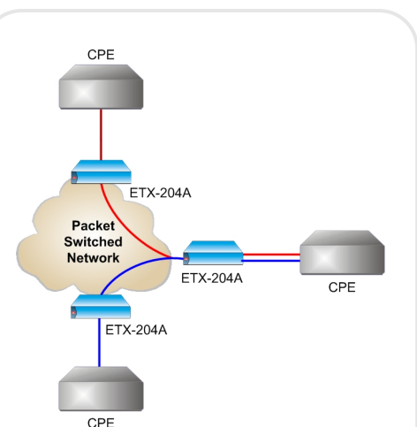
Figure 3. Ethernet Virtual Private Line
