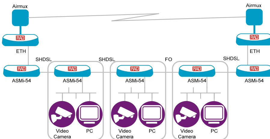
Figure 1. Daisy Chain over any Infrastructure for HDLC-Encapsulated Ethernet
